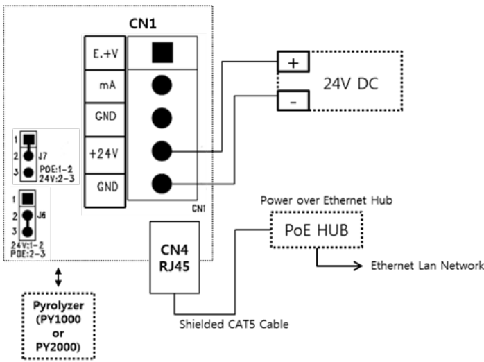
[Figure 12. Pyrolyzer Connection Configuration]
