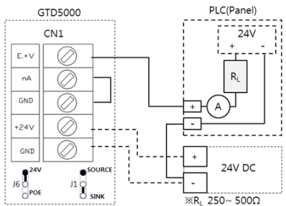
[Figure 9. 4-20mA Sink Configuration]
