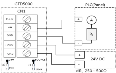
[Figure 7. 4~ 20mA Source Driver Configuration]
