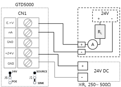
[Figure 8. 4-20mA Sink Configuration]
