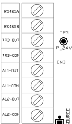
[Figure 10. CN3 Terminal Configuration]
