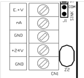
[Figure 6. CN1 Terminal Configuration]
