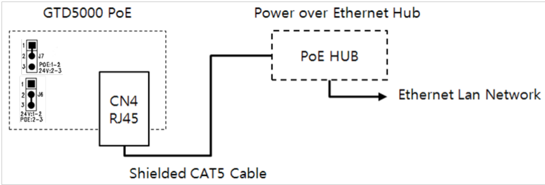
[Figure 11. PoE Configuration]
