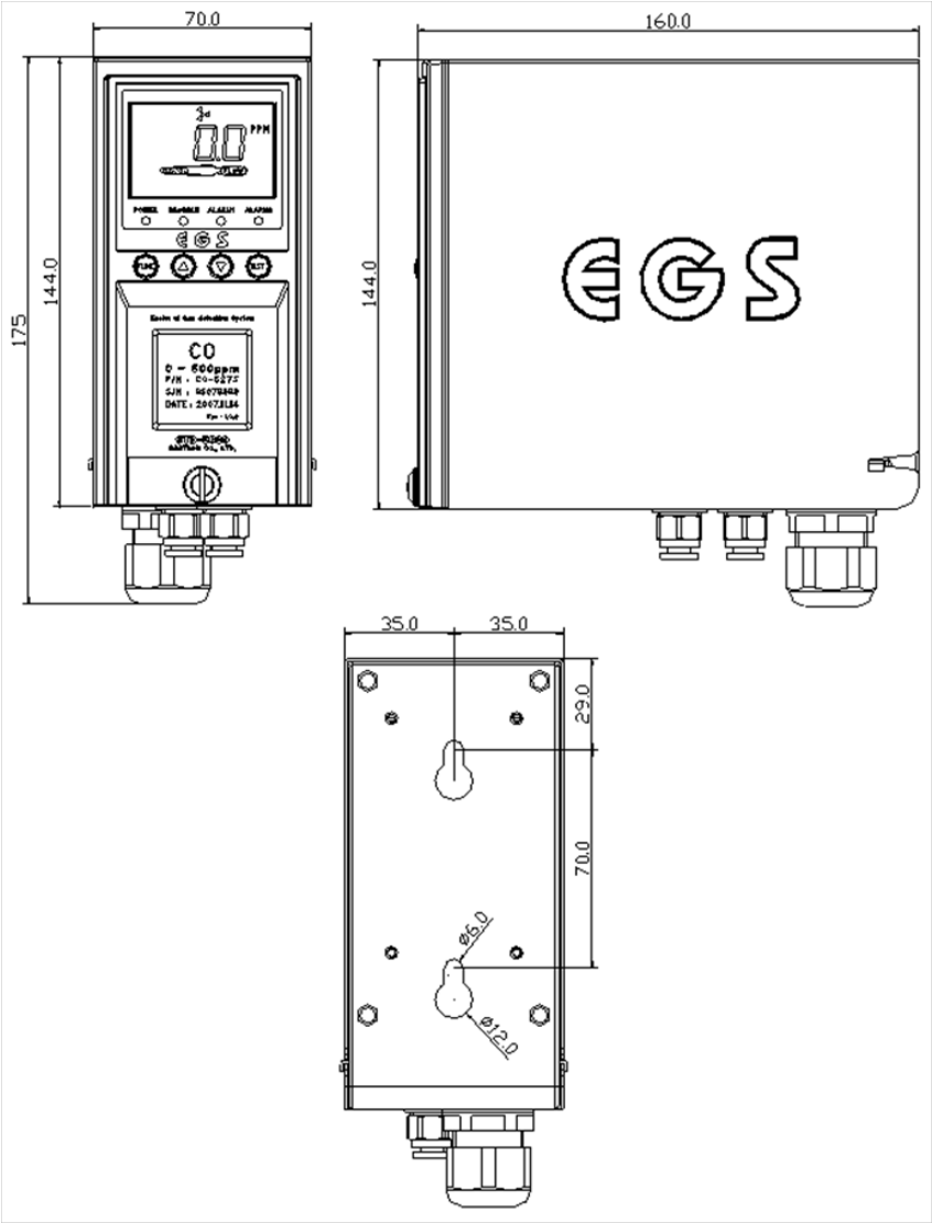
[Figure 14. GTD-5000 Dimension]
