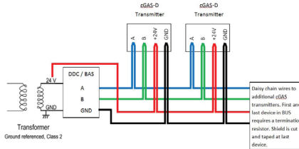
CGAS-D Connected to a BAS/DDC (4-wire VAC)
